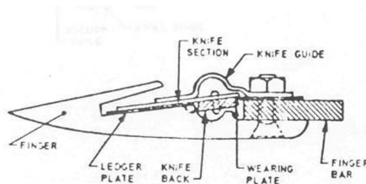
Cutter bar
