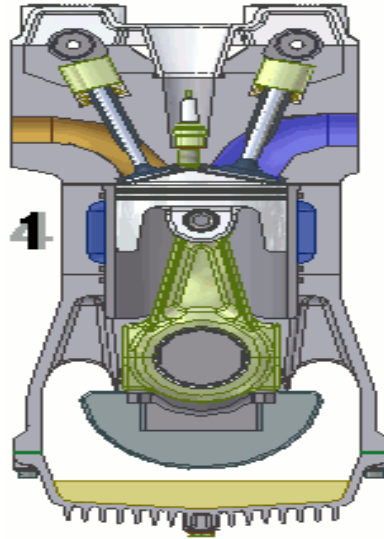
Four stroke cycle engine
