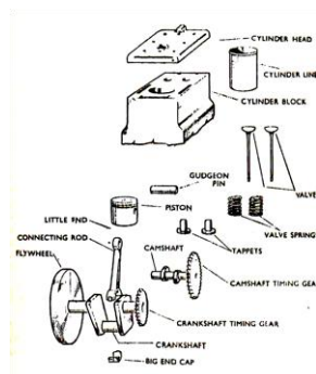
Engine components
