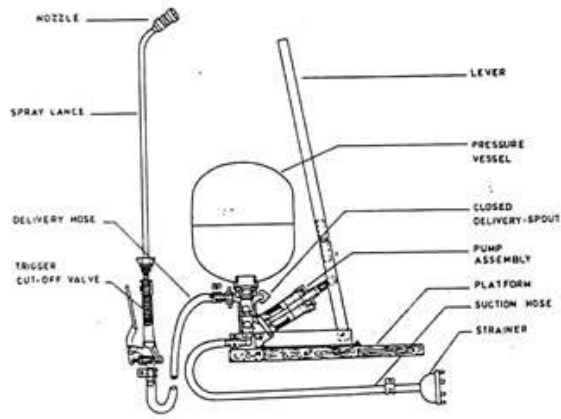
Rocker sprayer
