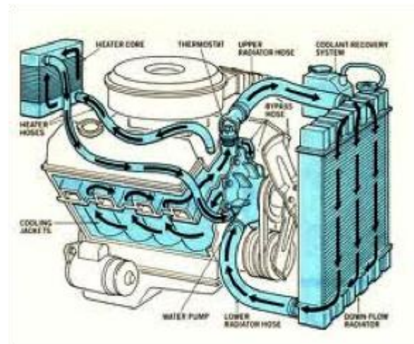
Forced Circulation cooling system- Water cooled engine
