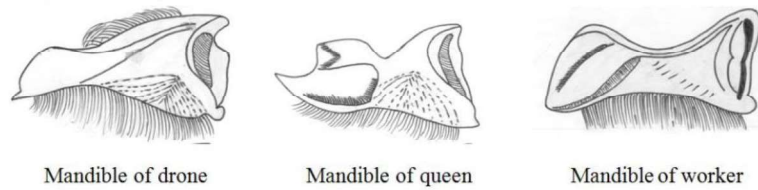
Figure 3.2 Mandibles of different castes of honey bees
